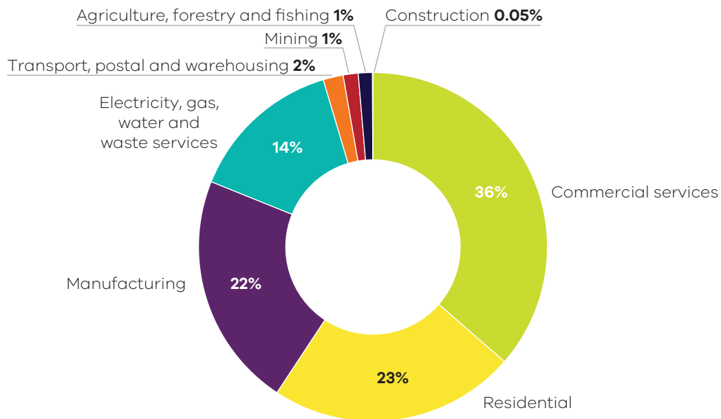
Figure 46: Scope 2 emissions by economic sector – Victoria, 2018
