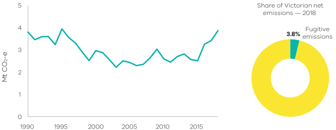
Figure 29: Emissions from fugitives – Victoria, 1990 to 2018
