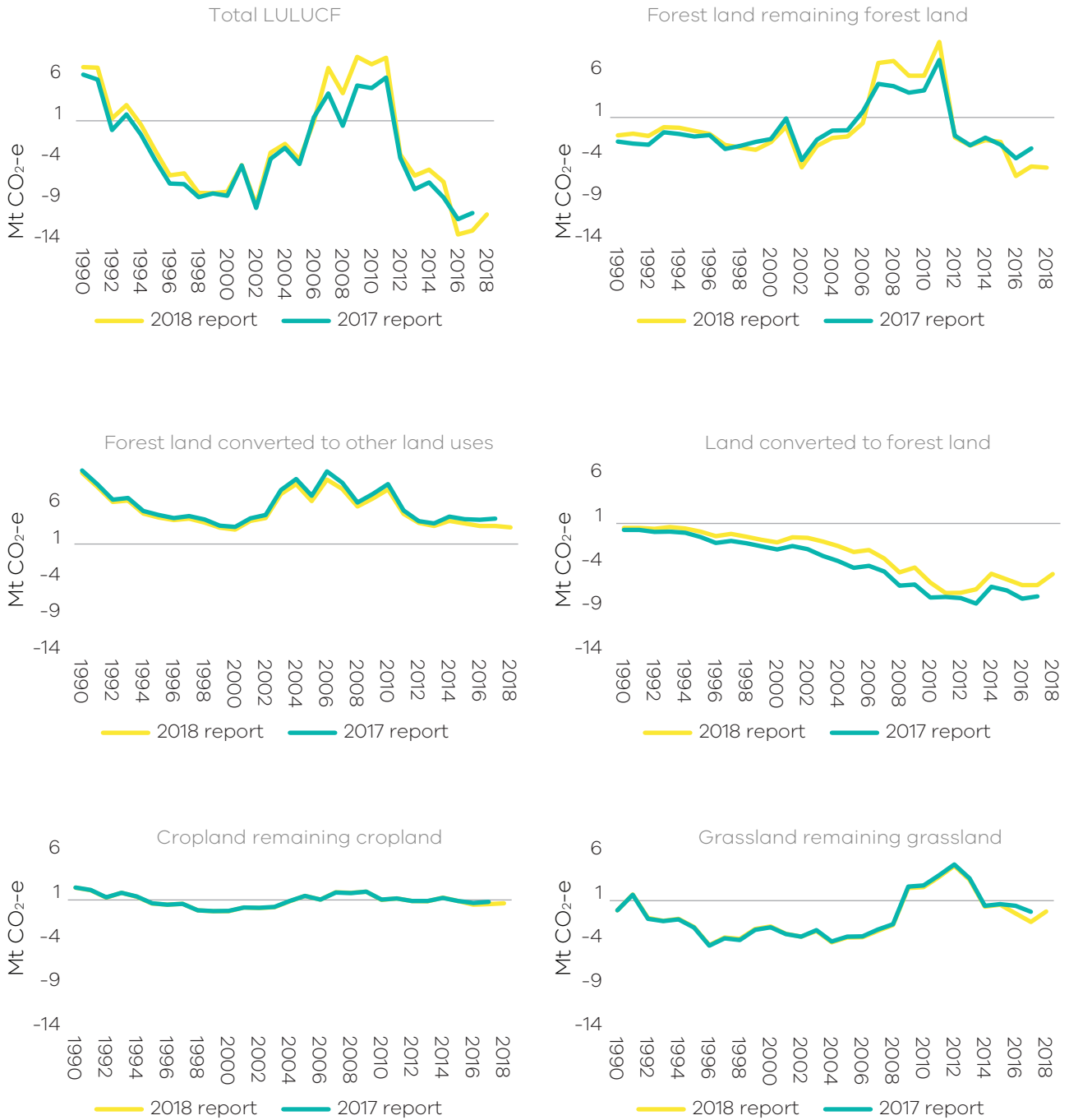
Figure 50: Emissions from Victoria’s main LULUCF sub-categories – comparison of 2017 and 2018 reports
