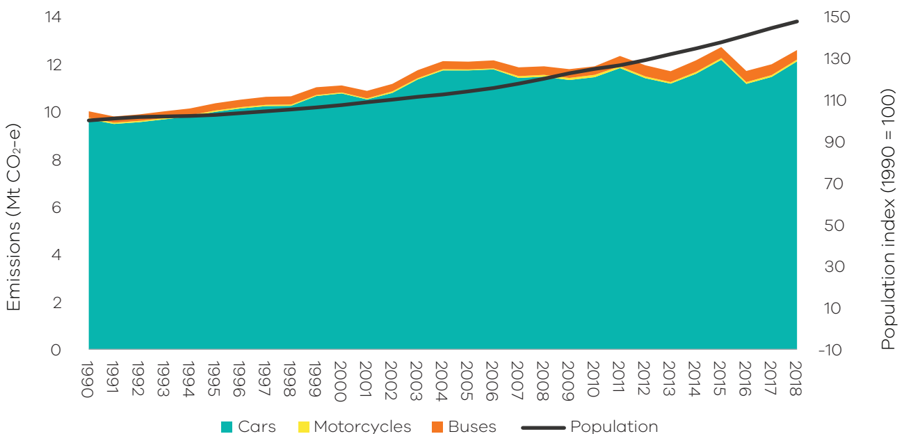
Figure 27: Trends in passenger motor vehicle emissions and population – Victoria, 1990 to 2018
