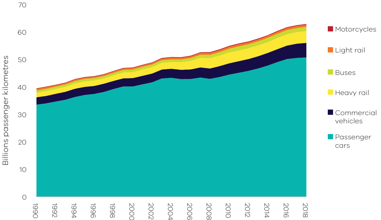
Figure 23: Total passenger kilometres travelled – Melbourne, 1990 to 2018
