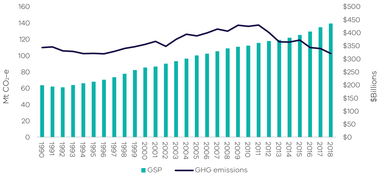
Figure 9: Greenhouse gas emissions and real GSP – Victoria, 1990 to 2018
