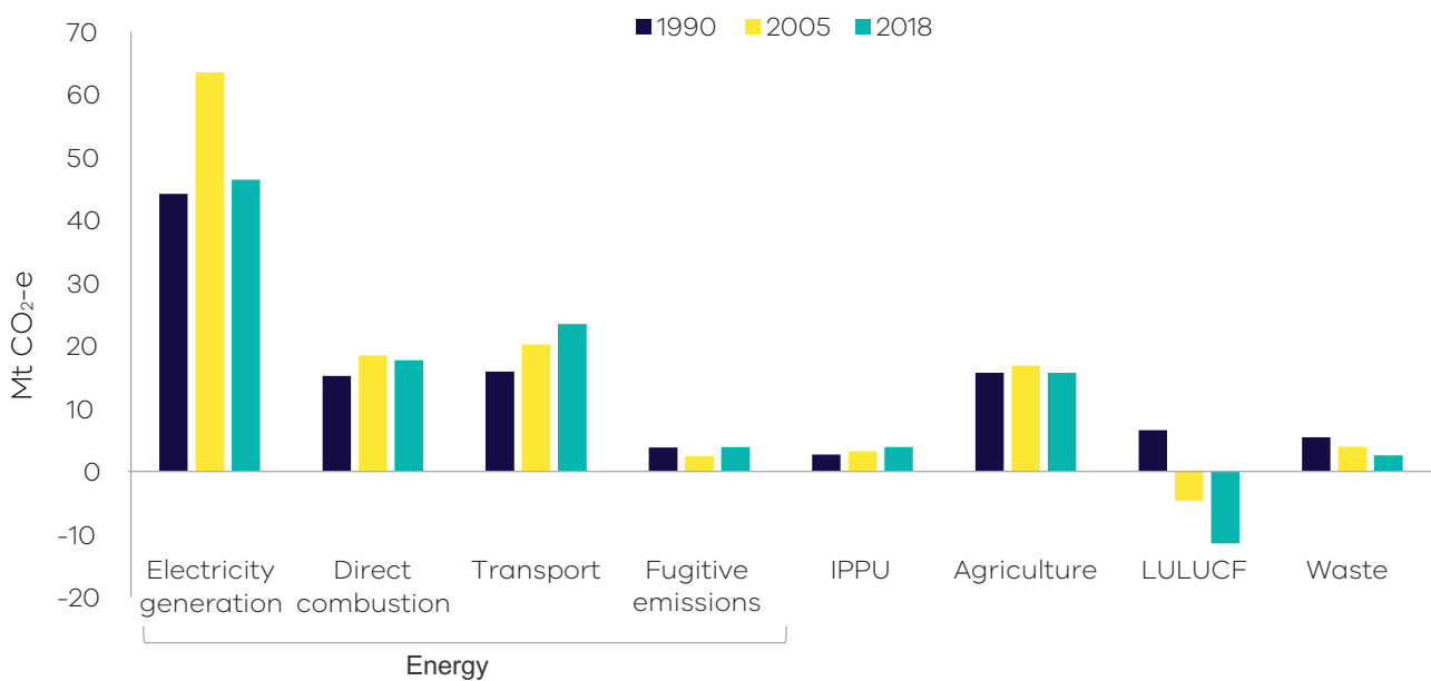
Figure 12: Emissions by sector – 1990, 2005 and 2018
