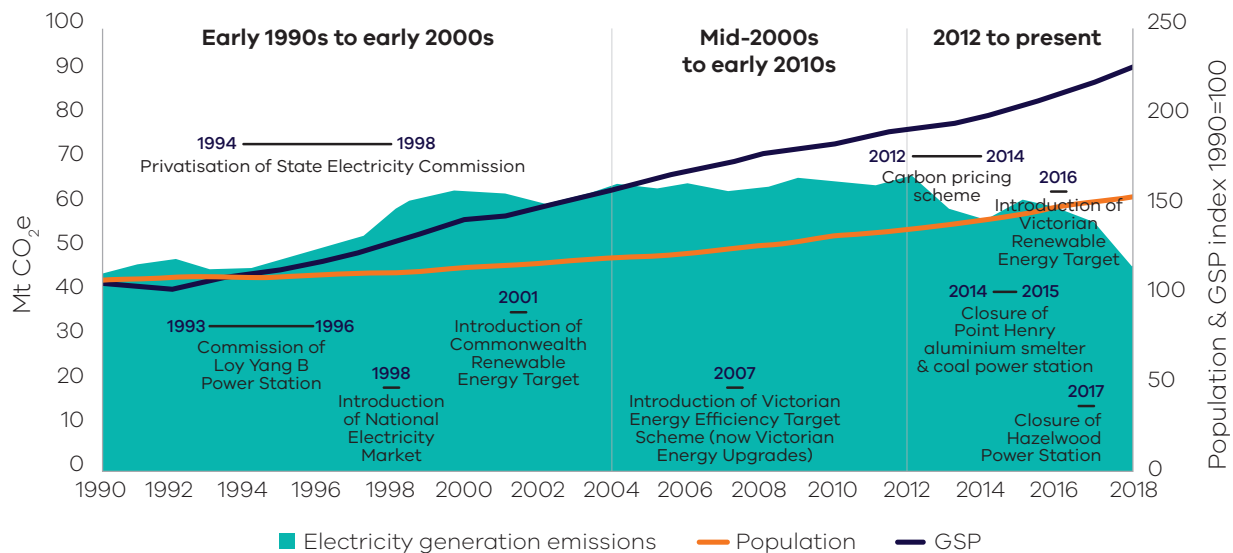
Figure 16: Emissions from electricity generation and trends in population and GDP
