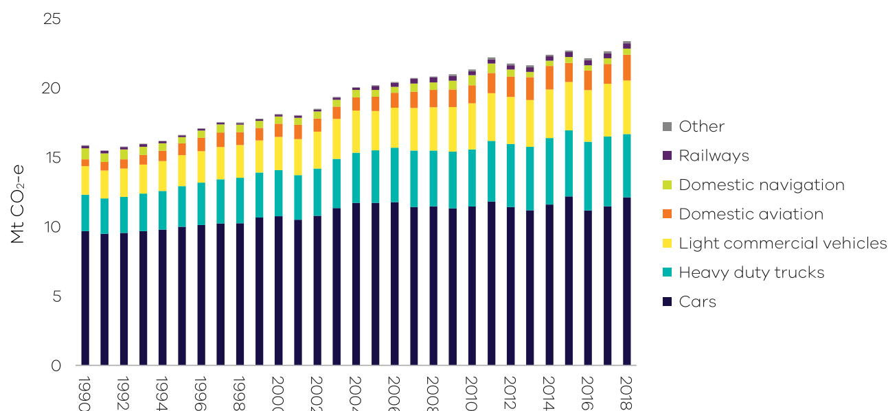
Figure 25: Emissions from transport sub-categories – Victoria, 1990 to 2018
