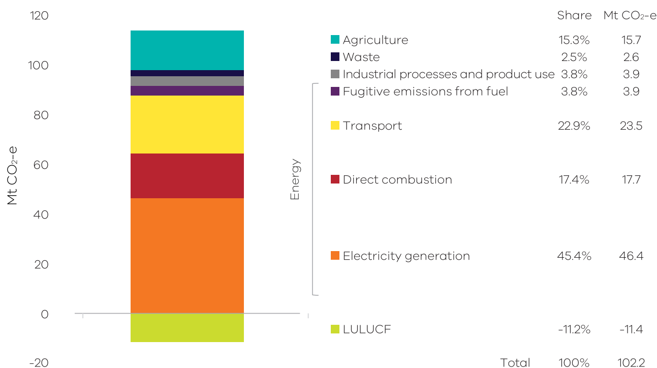
Figure 1: Victorian emissions by sector and energy sub-sector, 2018 2
